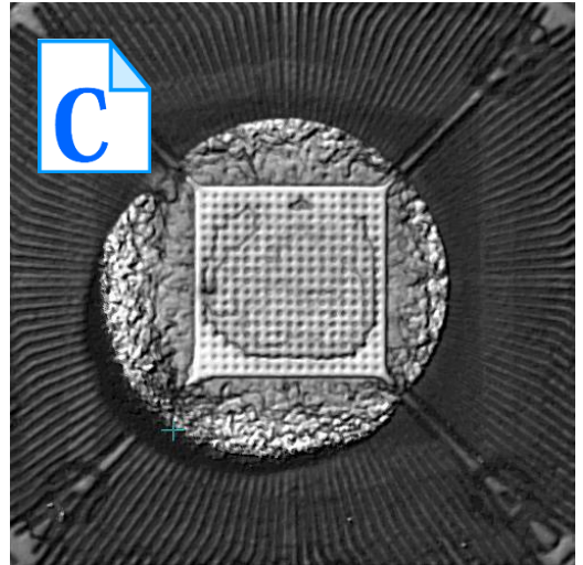
High Resolution C-Scan
