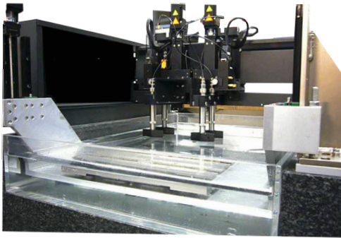
Multihead system with customized sample holder.
